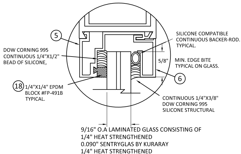
GLAZING DETAIL 2
