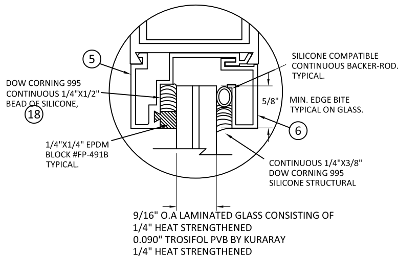
GLAZING DETAIL 1
